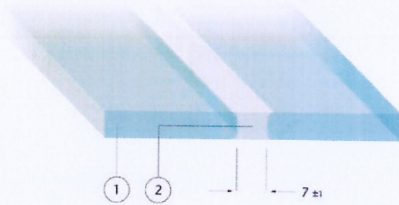
Butt-Joint Glazing Details
