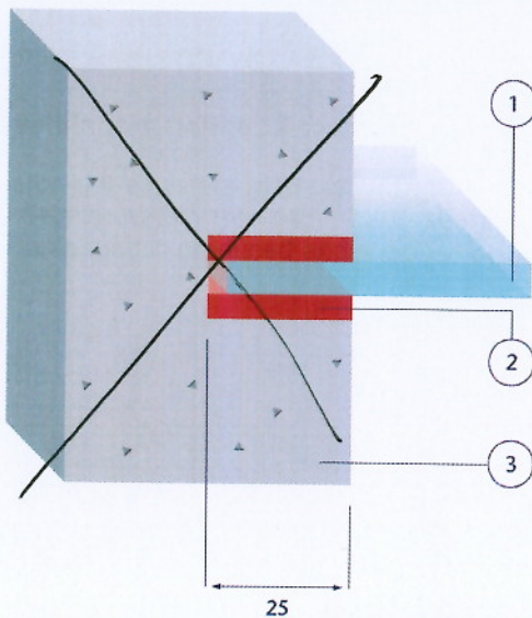
Alternative Perimeter Detail
